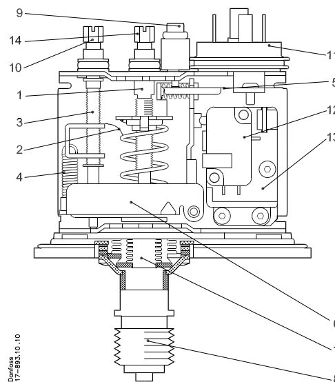
Simplified drawing of BCP control
