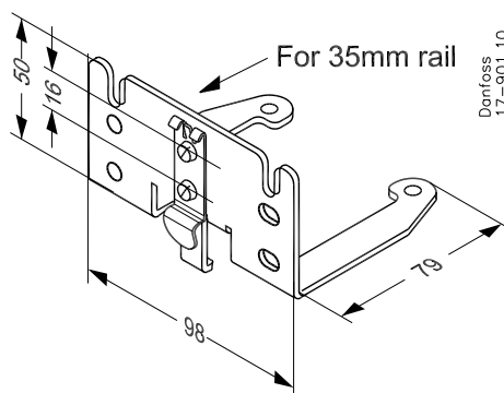
2. Mounting bracket for T 35 mm rail, code number 017B019
